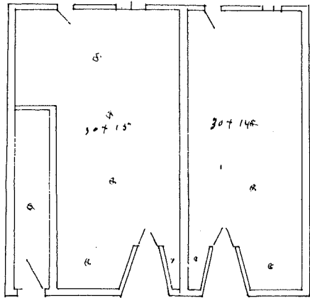
GROUND PLAN
