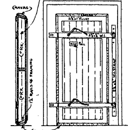
ELEVATION CHAMBER DOORS
