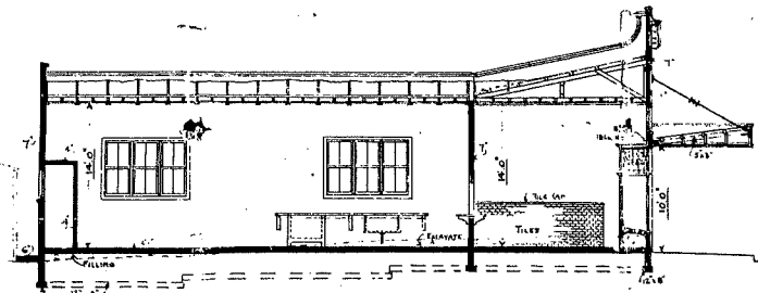
SECTION C.D.
