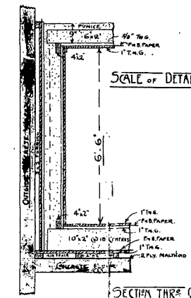
SECTION THROUGH CHAMBER
