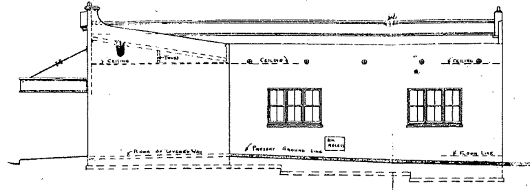
SIDE ELEVATION
