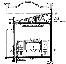
SECTION A.D.
